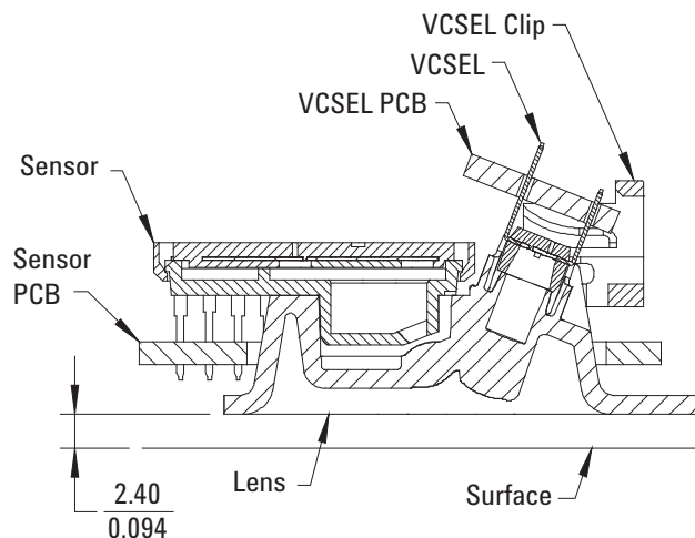
Figure 10. Distance from lens reference plane to surface
