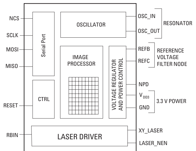
Figure 8. Block diagram of ADNS-6010 optical mouse sensor
