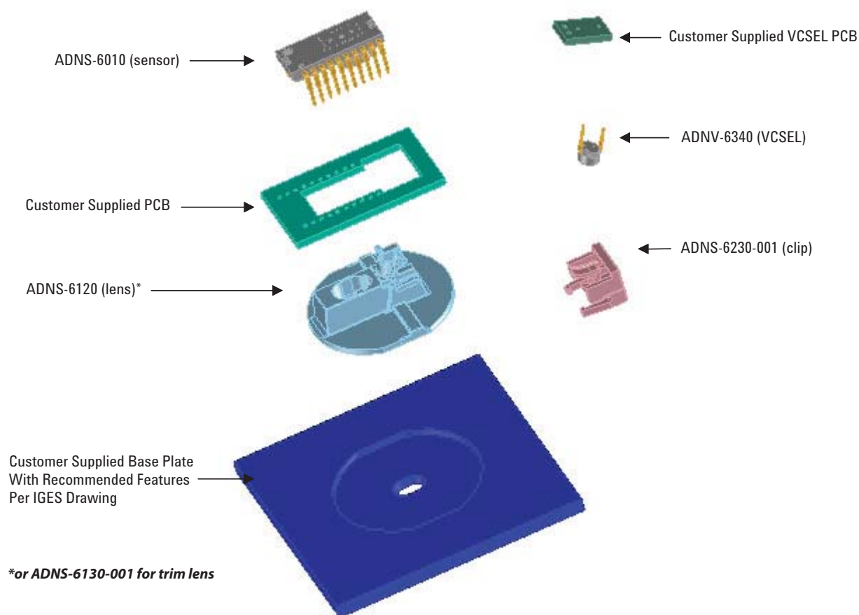
Figure 4. Exploded view drawing
